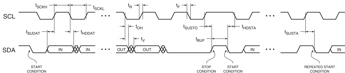
Figure 11-1. SMBus/I 2 C Timing Diagram
