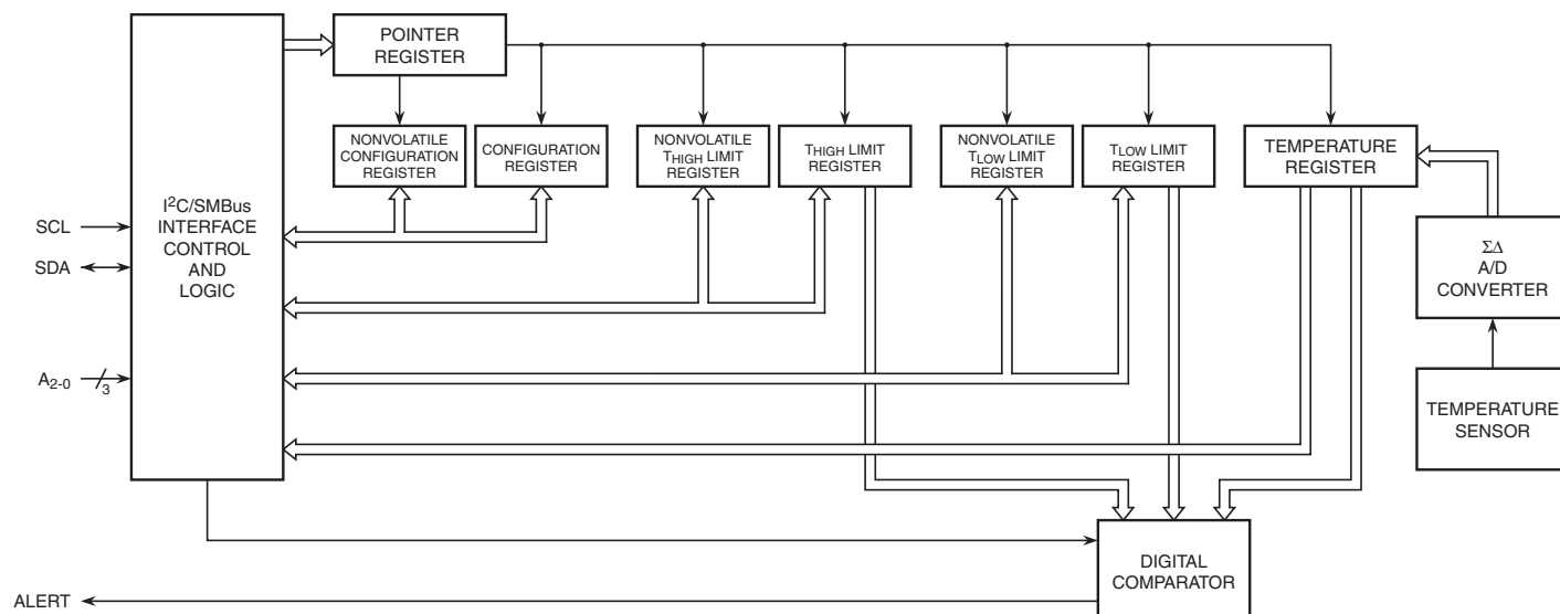
Figure 3-1. Block Diagram
