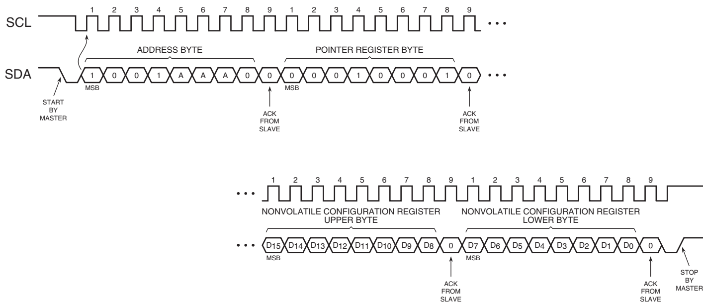
Figure 6-6. Write to Nonvolatile Configuration Register
