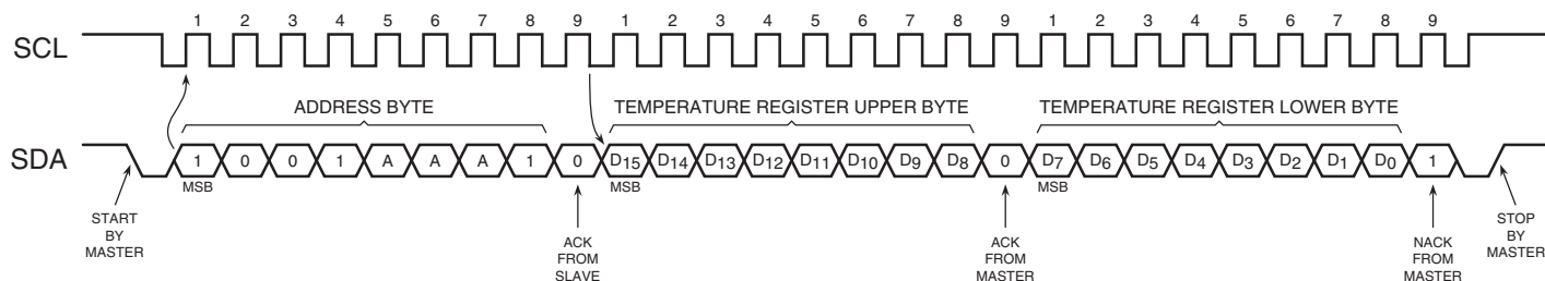
Figure 6-2. Read Temperature Register – 16 Bits
