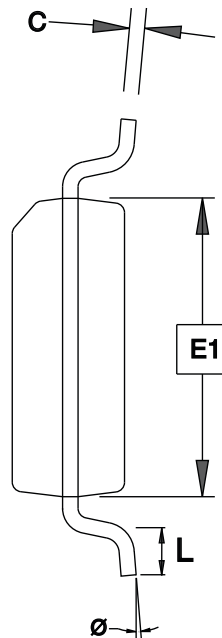
END VIEW
