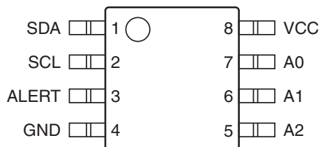
Figure 2-1. 8-SOIC (Top View)
