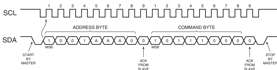
Figure 9-2. Copy Nonvolatile Registers to Volatile Registers
