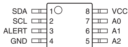
Figure 2-2. 8-MSOP (Top View)
