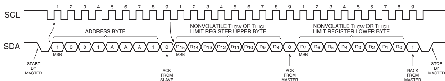
Figure 6-11. Read from Nonvolatile T LOW or T HIGH Limit Register
