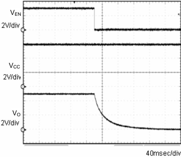
Fig.7 OFF sequence 2 C_o=1\mu F
