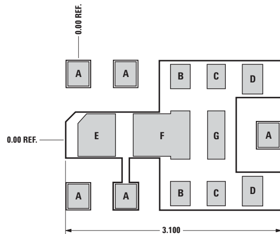
Combined PCB land pattern and stencil outline
