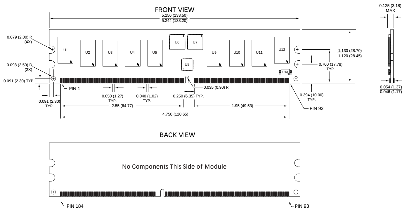
Figure 15: 184-PIN DIMM DDR Modules – Low-Profile
