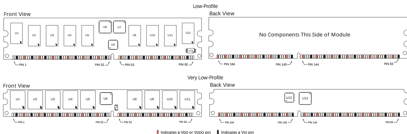
Figure 2: Pin Locations
