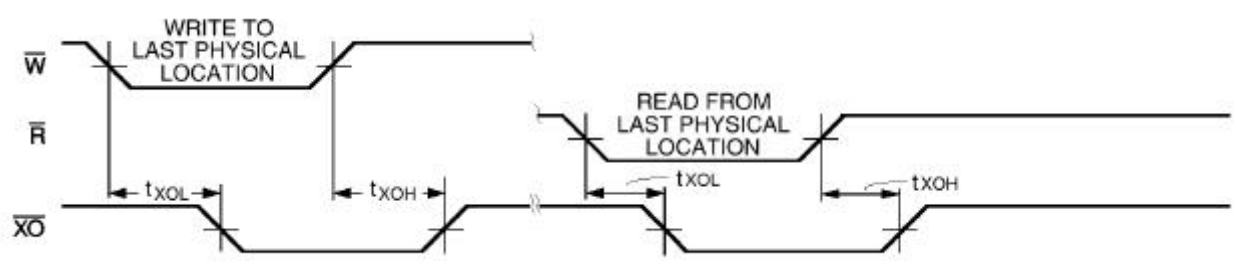
FIGURE 9. EXPANSION OUT
