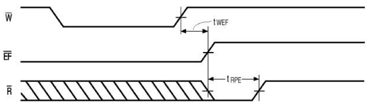
FIGURE 6. EMPTY FLAG TIMING
