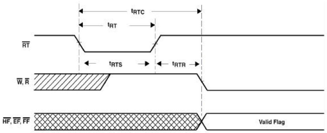
FIGURE 5. RETRANSMIT
