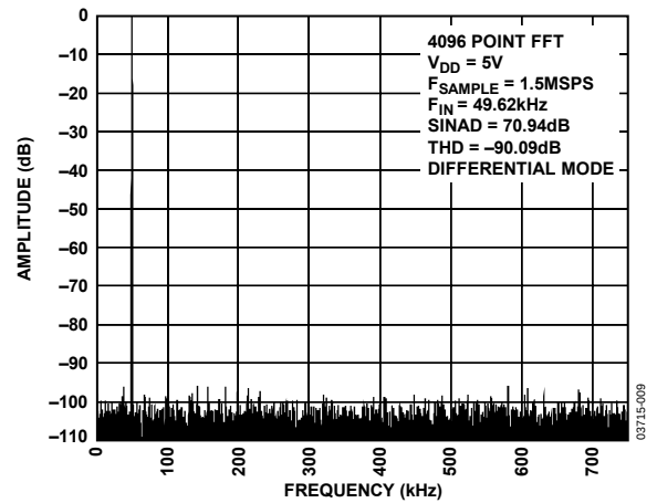
Figure 7. AD7938 FFT @ V_{DD} = 5\text{V}
