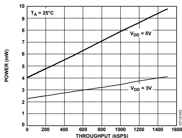
Figure 42. Power vs. Throughput in Normal Mode Using Internal Reference
