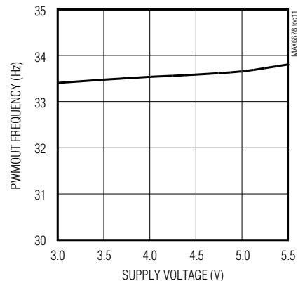
PWMOUT FREQUENCY vs. SUPPLY VOLTAGE
