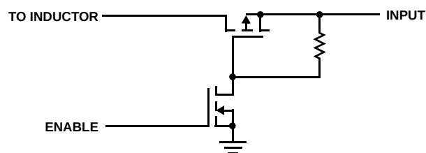
FIGURE 19. CIRCUIT TO DISCONNECT THE DC PATH OF BOOST CONVERTER
