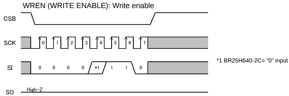
Figure 35. Write enable command
