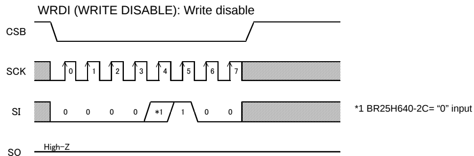
Figure 36. Write disable
