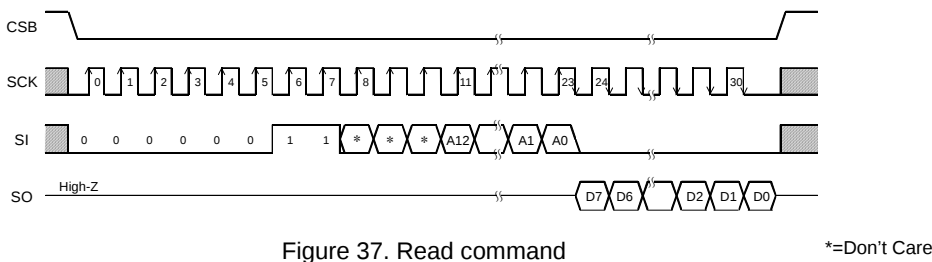
Figure 37. Read command
