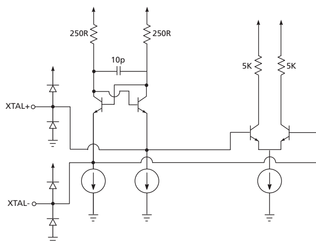
Figure 3-3: Crystal Input
