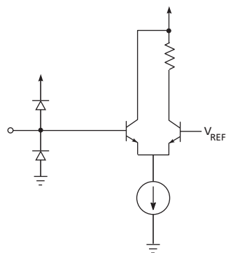
Figure 3-1: TTL Inputs
