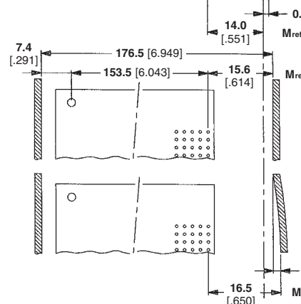
Subrack tolerances
