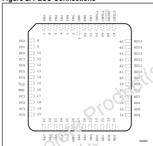
Figure 2. PLCC Connections
