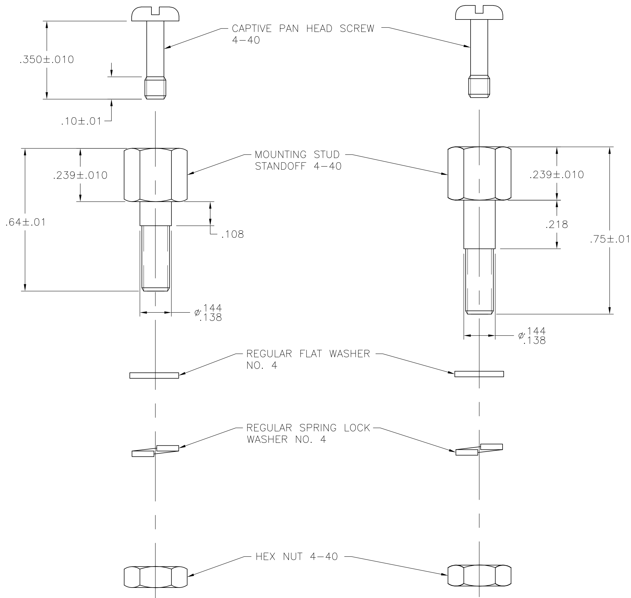
KIT P/N 5552568-1 VIEW A
