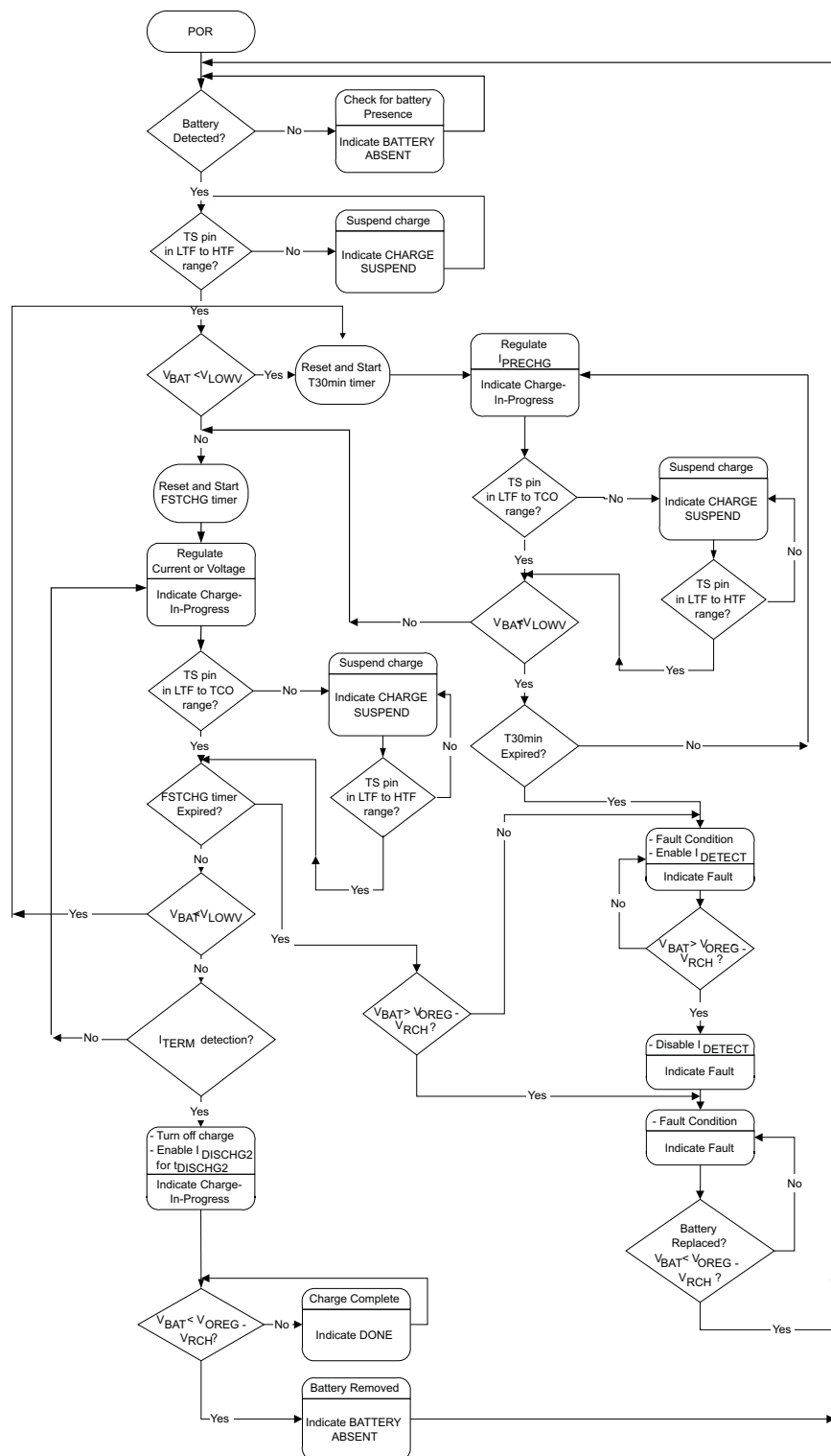
Figure 16. Operational Flow Chart
