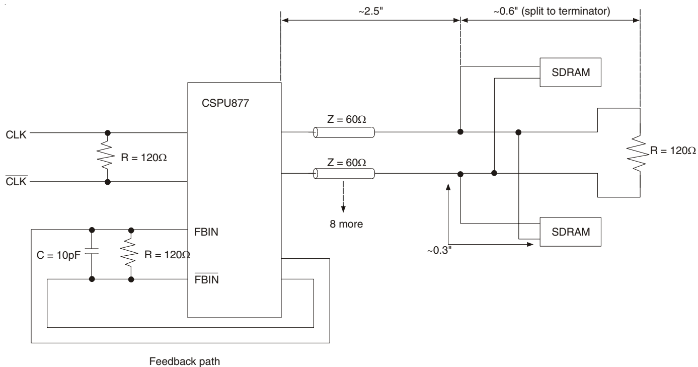
Clock Structure 1
