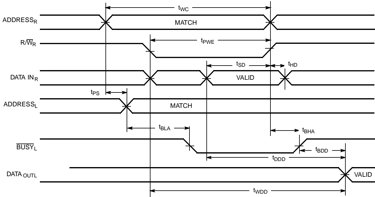
Timing Diagram of Read with \overline{\text{BUSY}} ( \text{M}/\overline{\text{S}}=\text{HIGH} ) [34]
