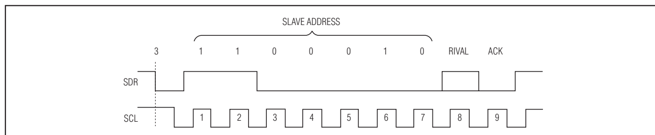
Figure 1. MAX2163 Slave Address Byte
