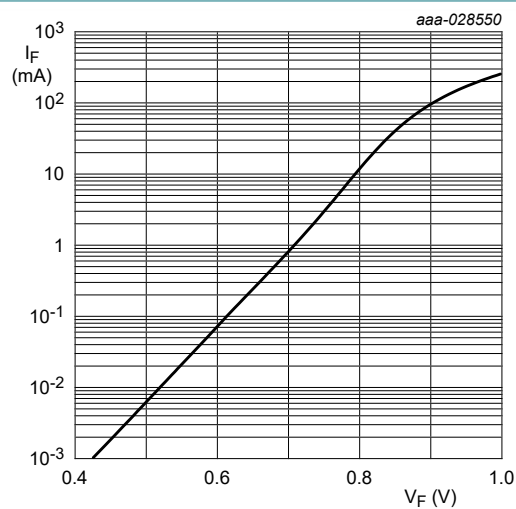
Fig. 2. BZX884-B/C2V4: Forward current as a function of forward voltage; typical values
