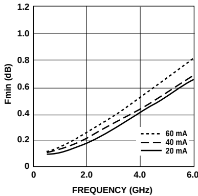
Figure 12. F_{min} vs. Frequency and Current at 4 V.
