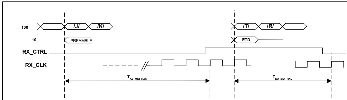
Figure 20: 10/100 to RGMII Receive Latency Timing
