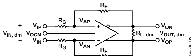
Figure 30. Circuit Definitions
