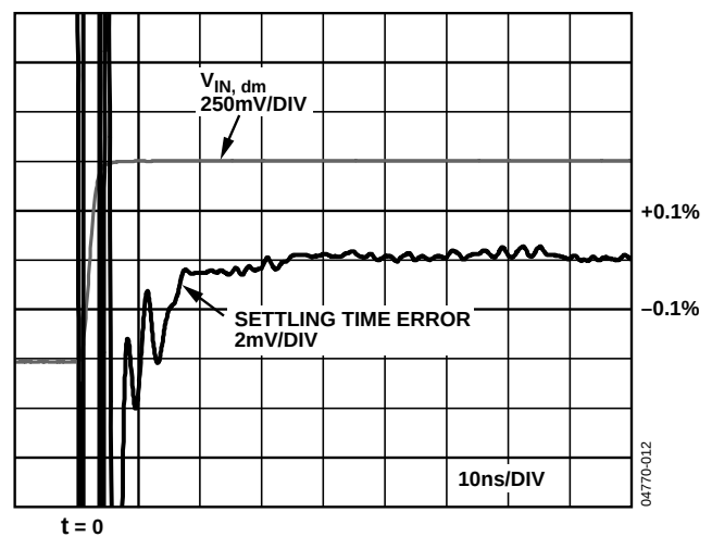
Figure 17. Settling Time (0.1%)
