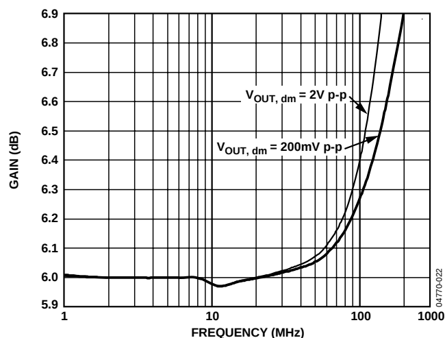
Figure 10. 0.1 dB Flatness
