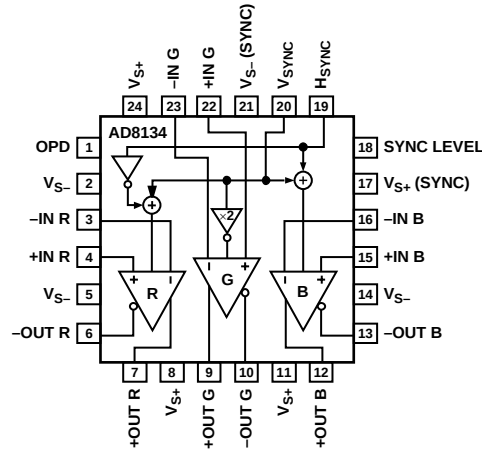
Figure 4. 24-Lead LFCSP
