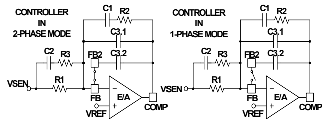
FIGURE 19. FB2 FUNCTION
