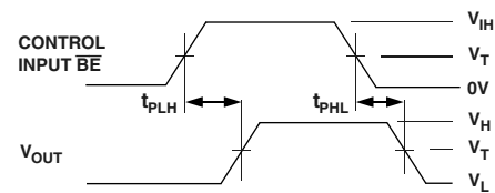
Figure 2. Propagation Delay
