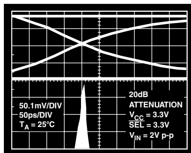
TPC 22. Jitter @ 1.244 Gbps, PRBS 31
