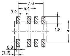
Mounting Dimensions (TOP VIEW) Tolerance: \pm 0.1 mm
