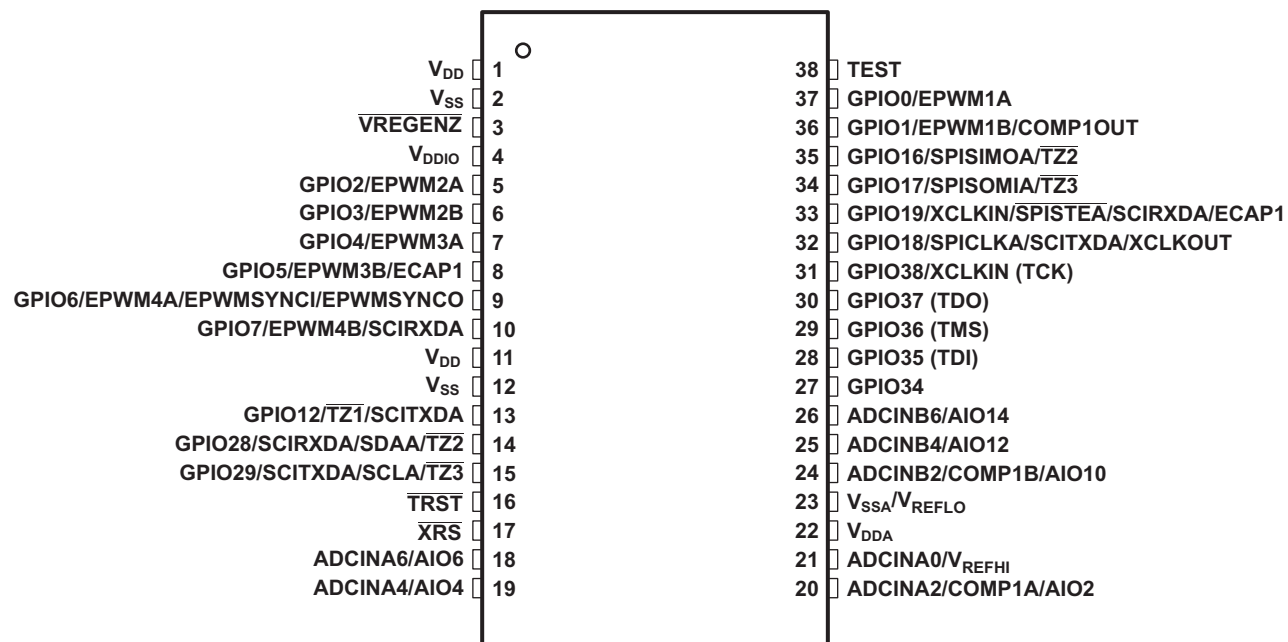
Figure 4-2. 2802x 38-Pin DA TSSOP (Top View)
