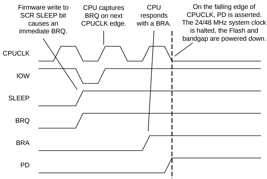
Figure 12-1. Sleep Sequence
