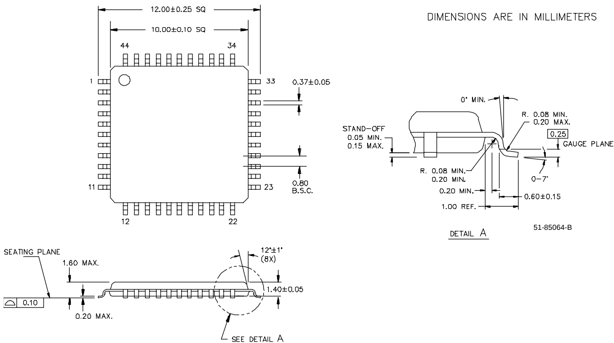
Figure 2-7. 44-Lead TQFP
