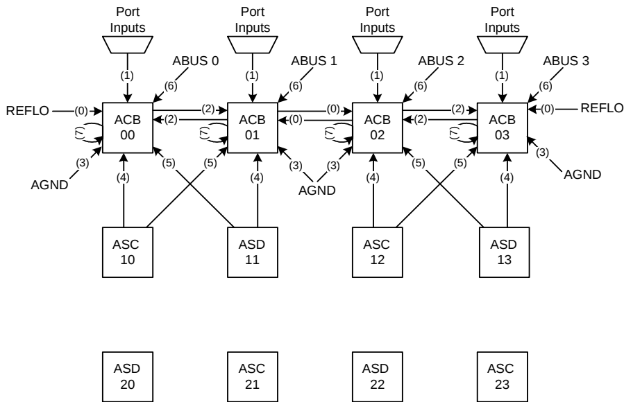
Figure 19-3. PMux Connections
