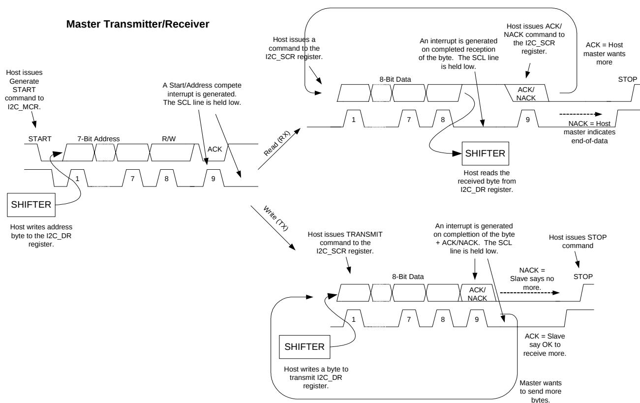
Figure 27-3. Master Operation
