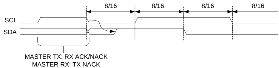
Figure 27-14. Master Restart Timing
