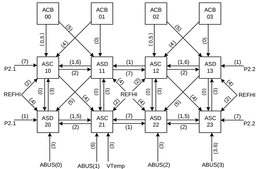
Figure 19-5. AMux Connections
