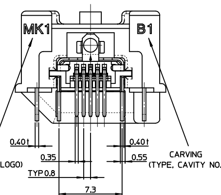
SECTION Z-Z
