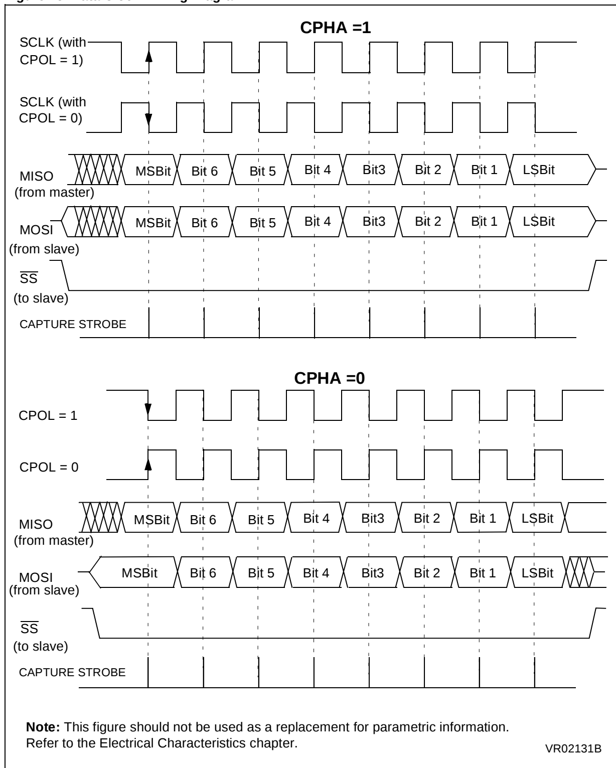
Figure 45. Data Clock Timing Diagram
