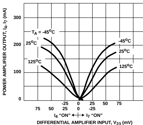
FIGURE 3B. CHARACTERISTIC WITH R_{10} IN CIRCUIT
