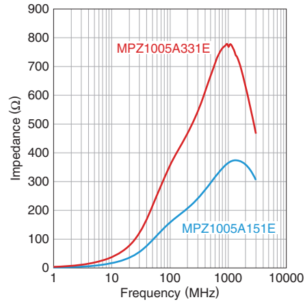
MPZ1005A-E series
