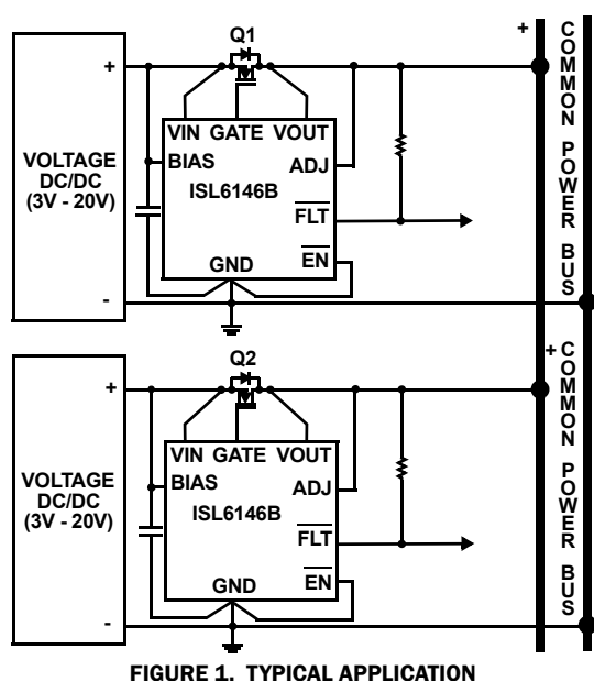
FIGURE 1. TYPICAL APPLICATION
