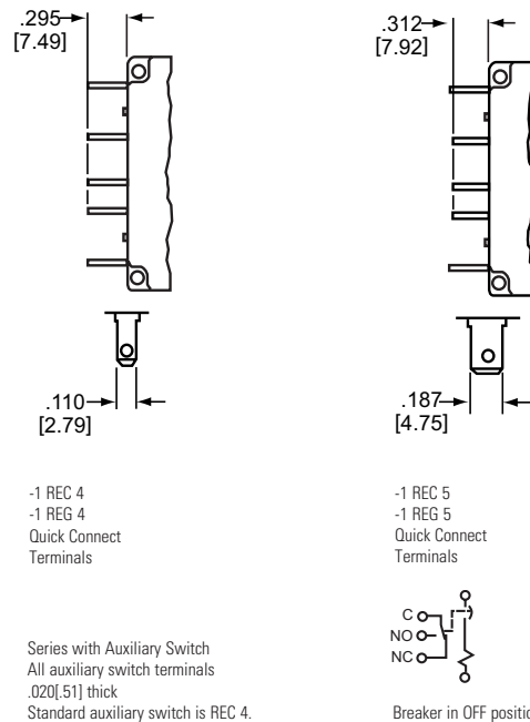
Auxiliary Switch
