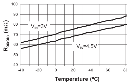
R_{DS(ON)} vs. Temperature
