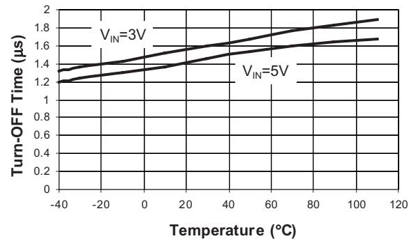
Turn-Off vs. Temperature
