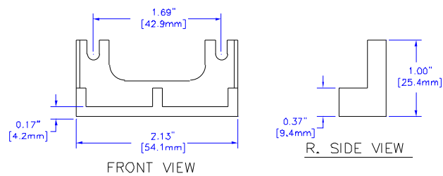
MOUNTING FEET DETAIL
