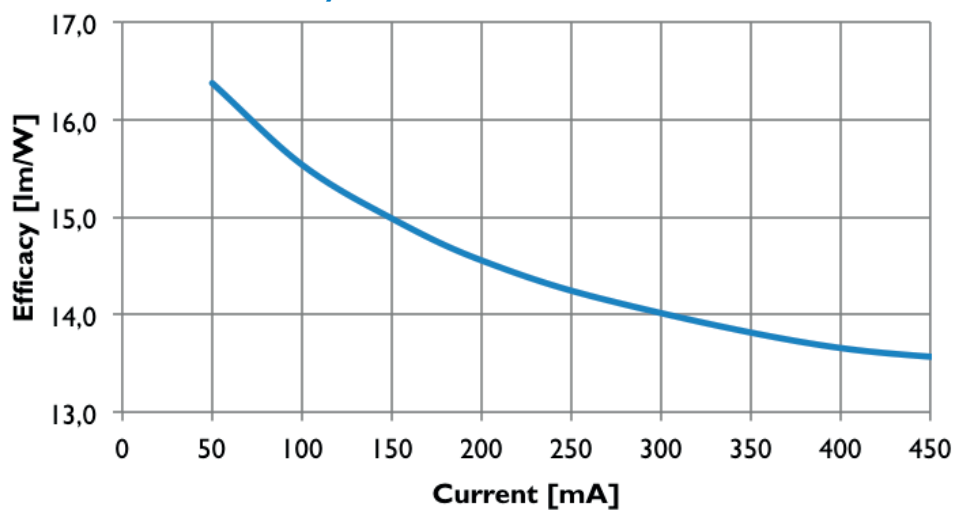
Luminous efficacy
