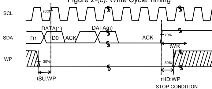
Figure 2-(d). WP Timing at Write Execution
