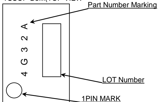
TSSOP-B8M(TOP VIEW)
