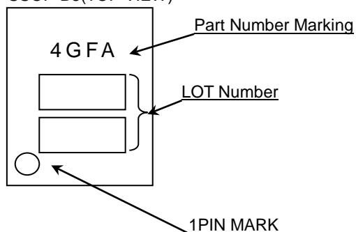
SSOP-B8(TOP VIEW)
