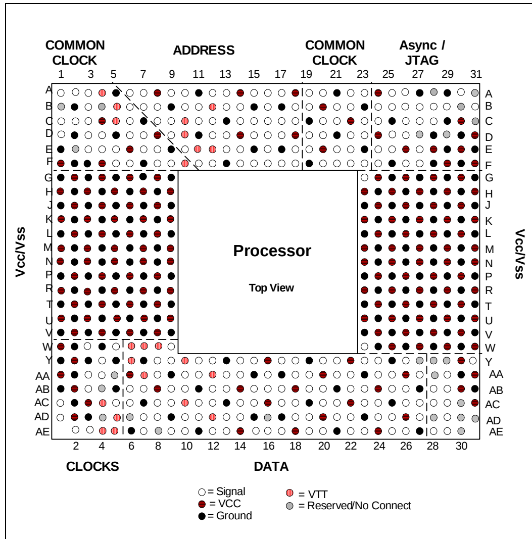
Figure 3-11. Processor Pin-Out Coordinates, Top View
