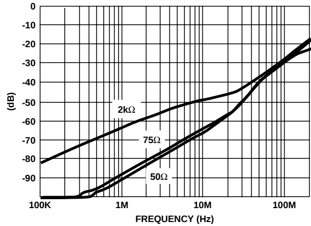
FIGURE 15. OFF ISOLATION
