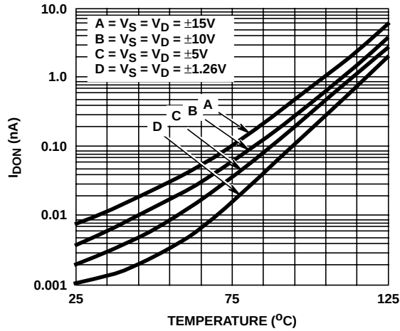
FIGURE 12. I_{\text{DON}} vs TEMPERATURE vs ANALOG INPUT
