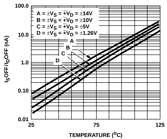
FIGURE 11. I_{SOFF}/I_{DOFF} vs TEMPERATURE vs ANALOG INPUT
