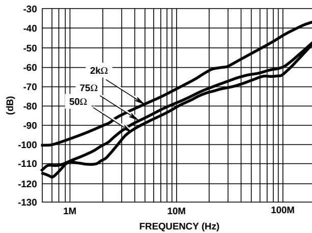
FIGURE 16. CROSSTALK
