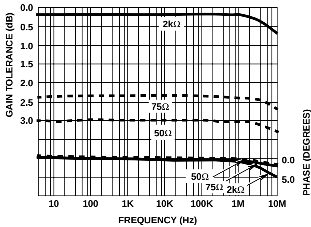
FIGURE 14. GAIN TOLERANCE
