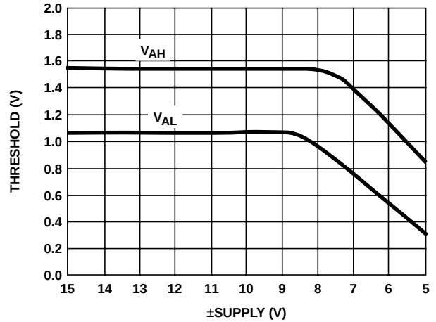
FIGURE 7. SWITCHING THRESHOLD vs \pm SUPPLY VOLTAGE
