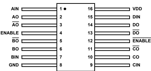
HS9-26C31RH, HS9-26C31EH (16 LD FLATPACK) CDFP4-F16 TOP VIEW
