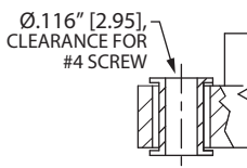
FLOATING BOBBIN (F)
