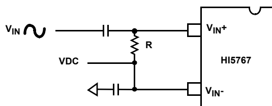
FIGURE 18. AC COUPLED SINGLE ENDED INPUT
