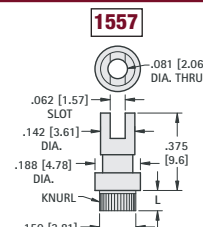
Staking Tool 1557-TL
