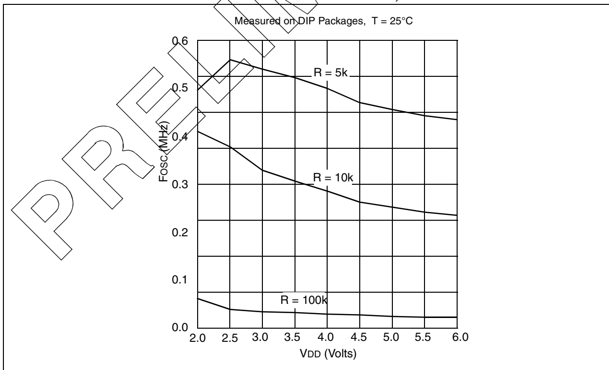
FIGURE 12-4: TYPICAL RC OSCILLATOR FREQUENCY vs. V_{DD} , C_{EXT} = 300\text{ pF}
