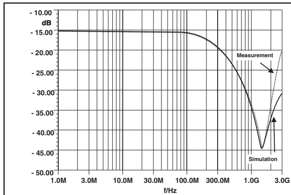
Figure 3. S21 (dB) attenuation measurement and Aplac simulation
