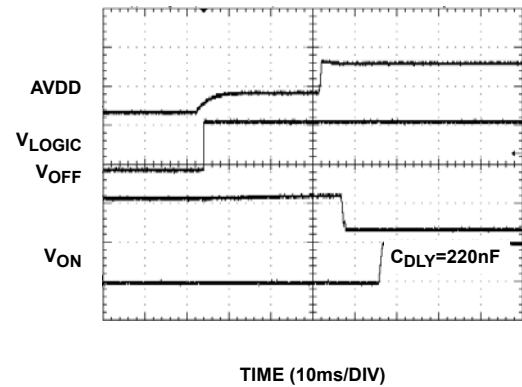
FIGURE 14. START-UP SEQUENCE
