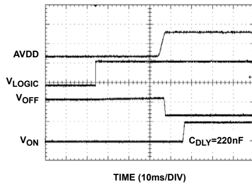
FIGURE 15. START-UP SEQUENCE
