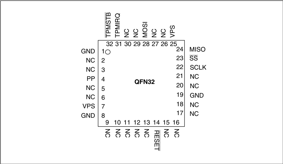
Figure 3. VQFN32 pinout
