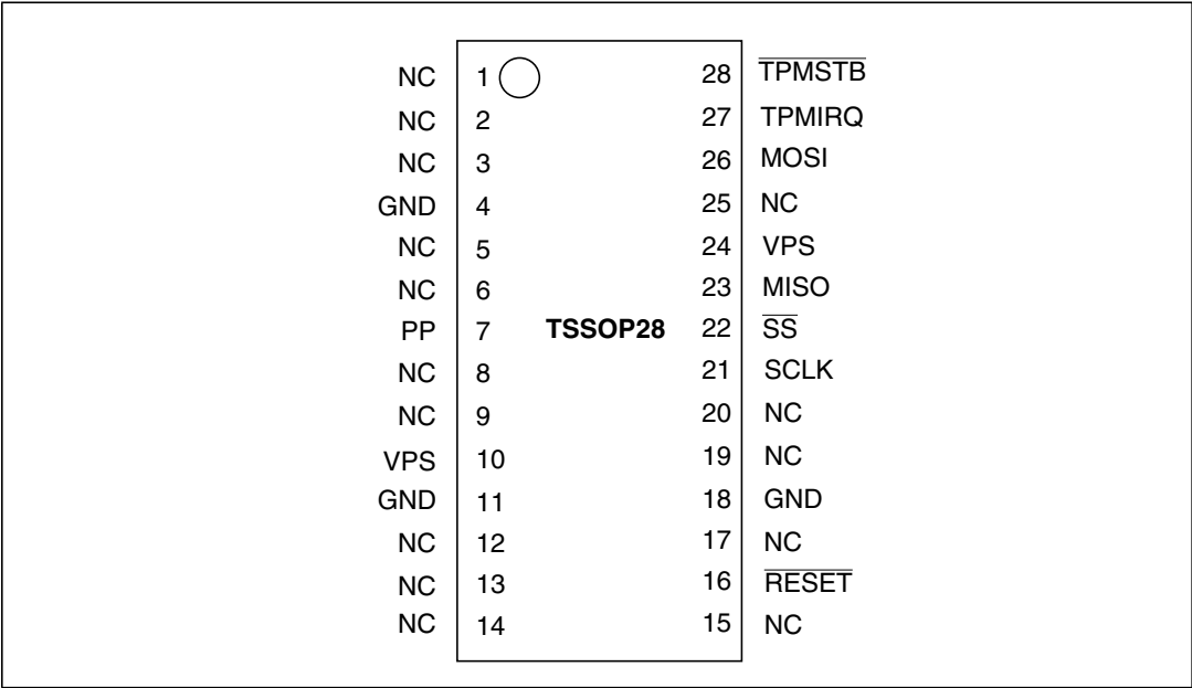
Figure 2. TSSOP28 pinout
