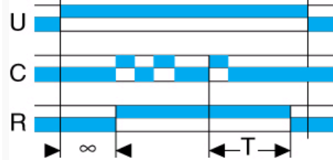
Function N - 1 relay output
