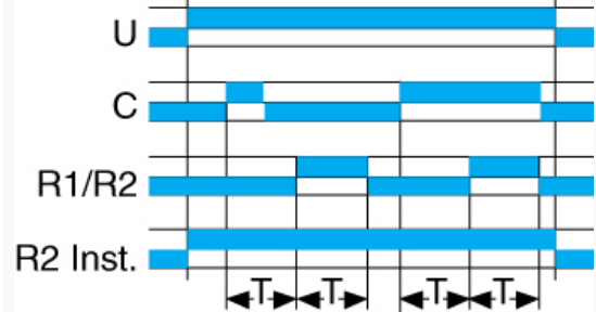
Function Ah - 1 relay output
