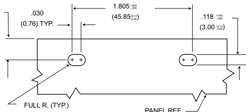
Figure 3 Edgeboard Mounting
