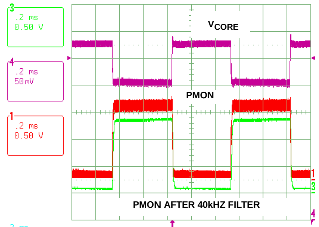
FIGURE 27. VID = 1.15V, LOAD TRANSIENT OF 0A TO 36A WITH INTEL \circledR VTT TOOL, 1kHz REPETITION RATE, 50% DUTY CYCLE, TR = 56
