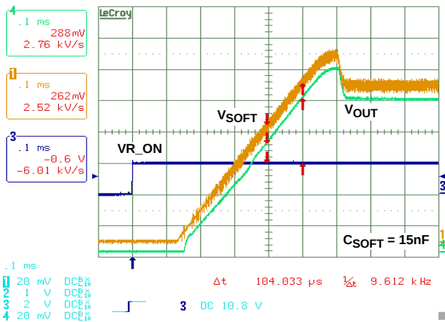
FIGURE 8. SOFT-START WAVEFORM SHOWING SLEW RATE OF 2.5mV/ \mu s AT VID = 1V, I_{LOAD} = 10A
