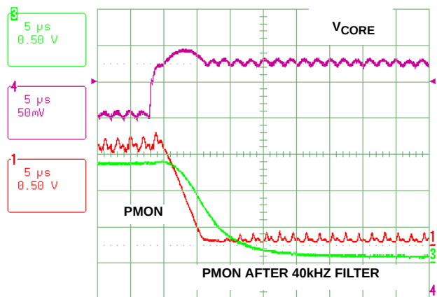
FIGURE 28. VID = 1.15V, LOAD RELEASE FROM 36A TO 0A WITH INTEL \circledR VTT TOOL, 1kHz REPETITION RATE, 50% DUTY CYCLE, TR = 56
