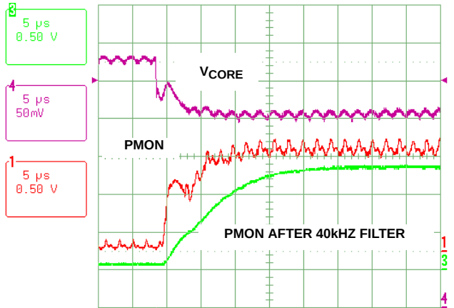
FIGURE 29. VID = 1.15V, LOAD APPLICATION FROM 0A TO 36A WITH INTEL \circledR VTT TOOL, 1kHz REPETITION RATE, 50% DUTY CYCLE, TR = 56
