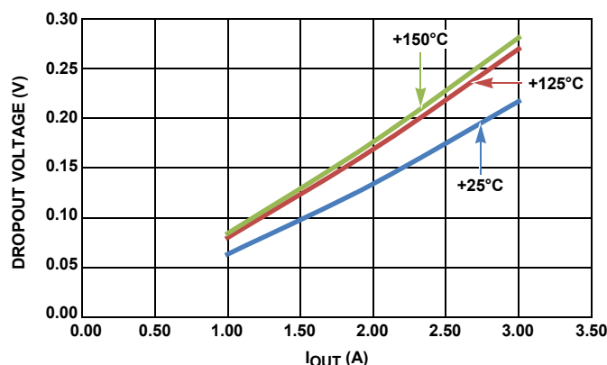
FIGURE 2. DROPOUT vs I OUT
